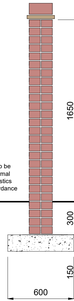
SECTION
